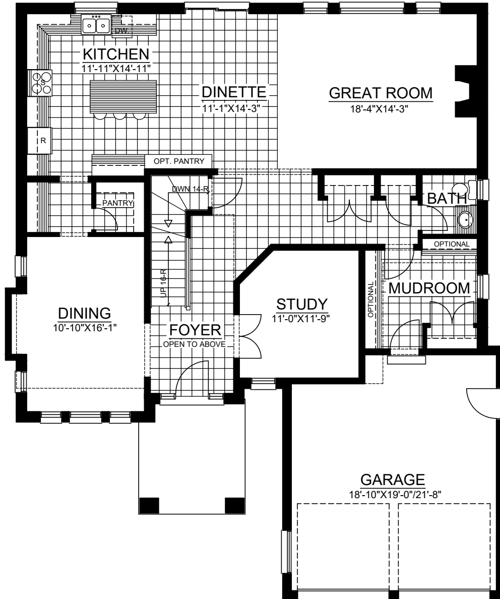
"MADISON" II FIRST FLOOR PLAN APPROX. 1541 SQ FT TOTAL APPROX. - 2870 SQ FT.
