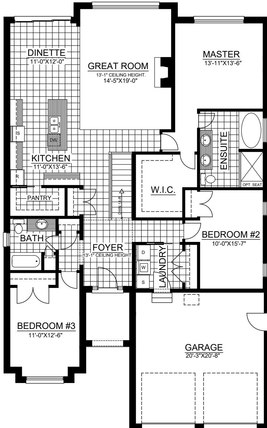
"STAPLETON" MAIN FLOOR PLAN TOTAL APPROX.- 2011 SQ FT.
