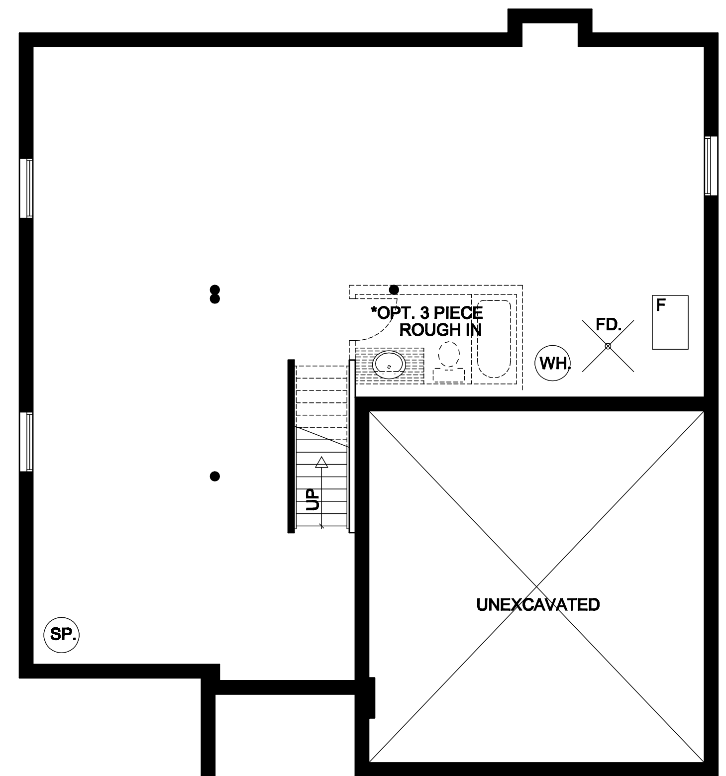
THE "PRESCOTT" FOUNDATION PLAN APPROX. 2140 SQ. FT.
