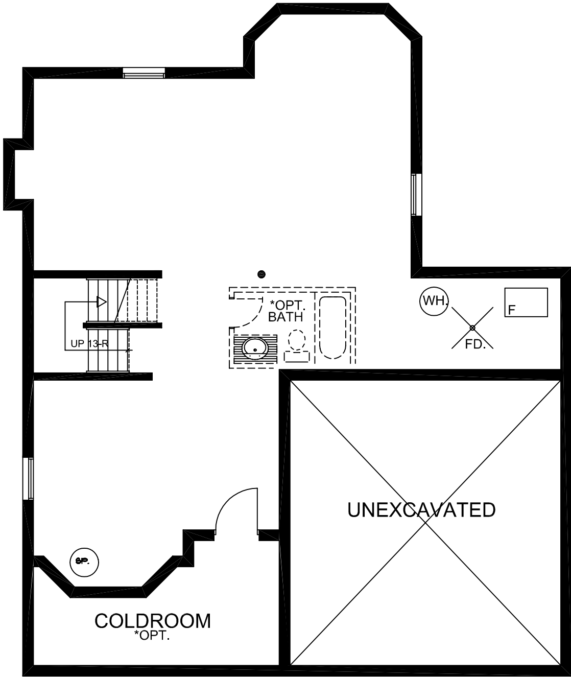
LAURENTIAN FOUNDATION PLAN APPROX. - 2014 SQ. FT.
