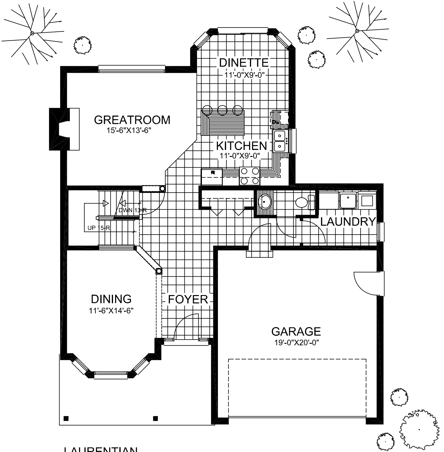
LAURENTIAN FIRST FLOOR PLAN APPROX. - 2014 SQ. FT.
