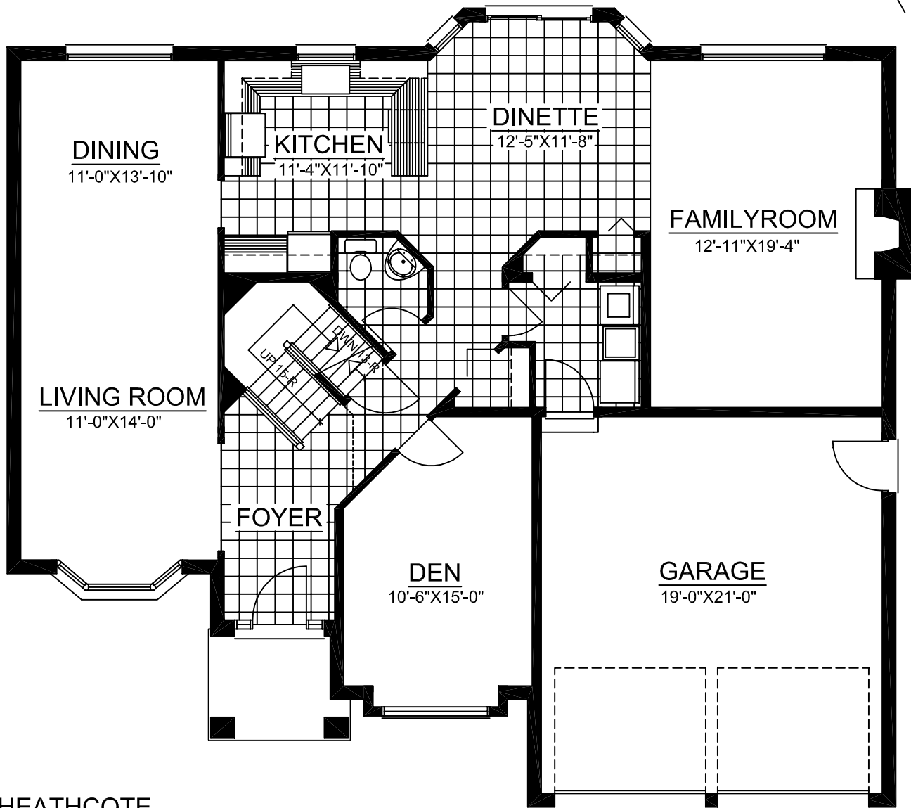
HEATHCOTE FIRST FLOOR PLAN APPROX. - 2509 SQ. FT.
