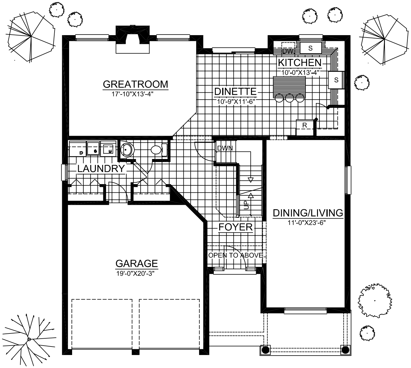
ACADIA MAIN FLOOR PLAN TOTAL APPROX. 2496 SQ FT.
