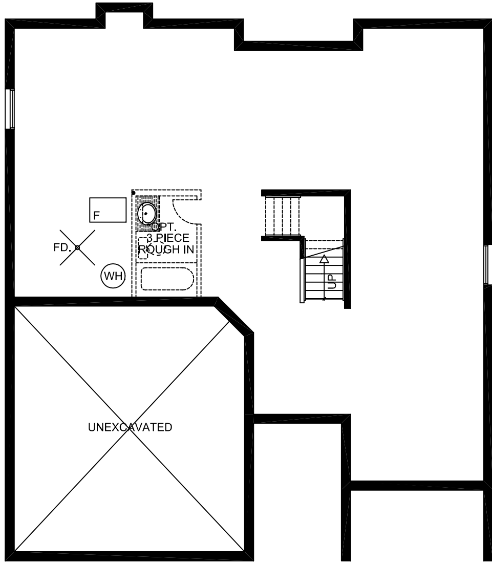
ACADIA FOUNDATION PLAN TOTAL APPROX. 2496 SQ FT.
